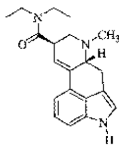
LSD
